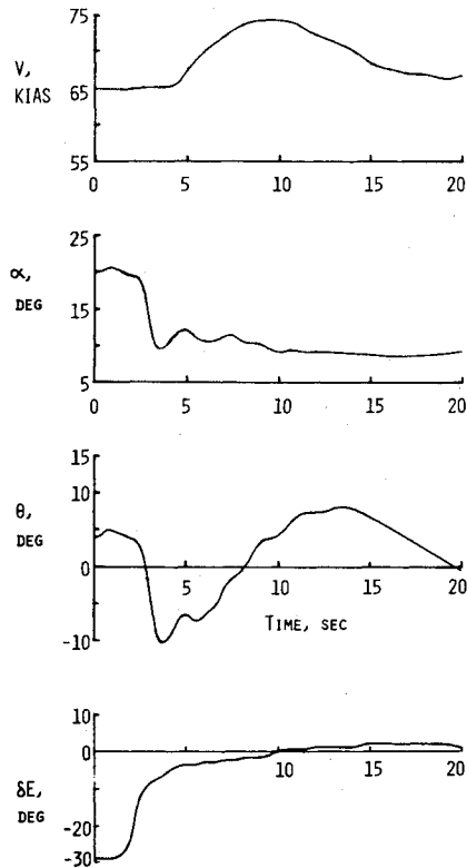
Fig. 14 ARA stall recovery.
