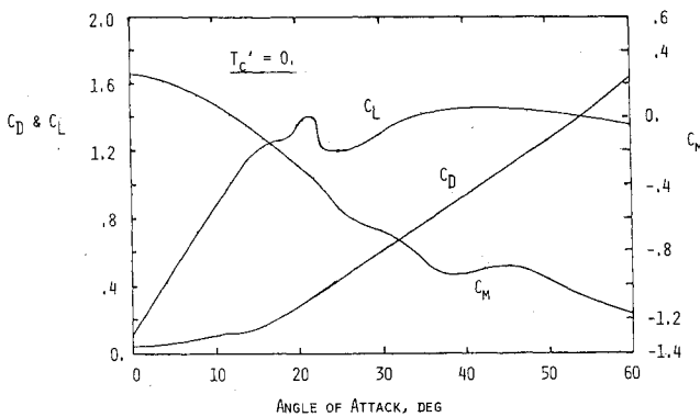
Fig. 3 Combined static longitudinal model (zero thrust).
