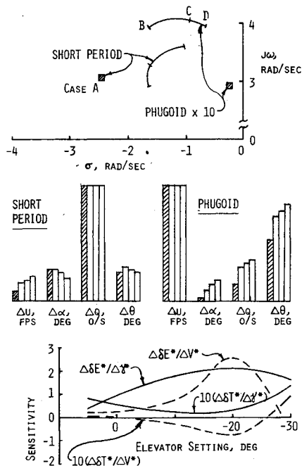
Fig. 9 Survey of stability and control characteristics for the power-off flight paths.
