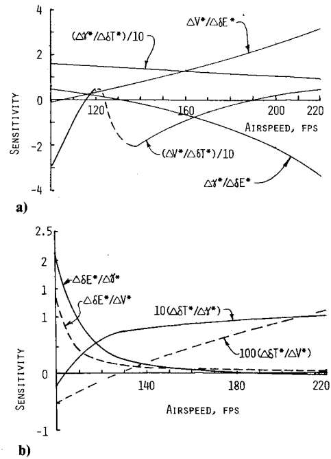
Fig. 7 Linear trim sensitivities as functions of airspeed. Altitude = 2286 m (7500 ft).
