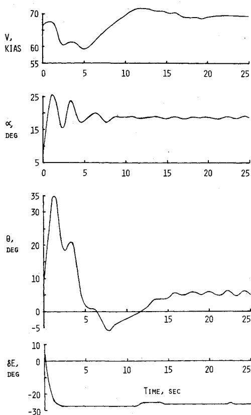
Fig. 16 Abrupt ARA stall. Starting altitude = 2438 m (8000 ft).
