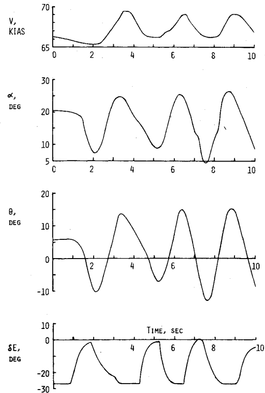
Fig. 15 Effects of elevator pumping in the ARA stall.
