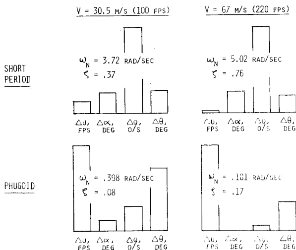
Fig. 6 Eigenvector magnitudes at two trim airspeeds. Altitude = 2286 m (7500 ft).
